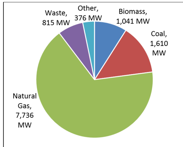
Figure II-4: Existing Commercial CHP Capacity by Fuel Class 37
